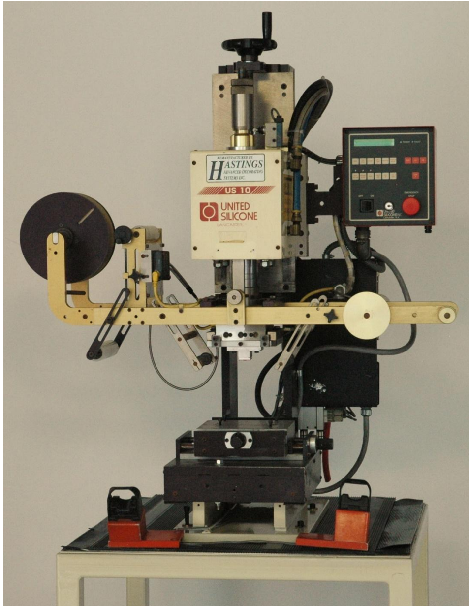
MODEL US 10, ONE TON HEAT TRANSFER PRESS. OPTIONAL X , Y TABLE AVAILABLE REMANUFACTURED BY HASTINGS ADS.
